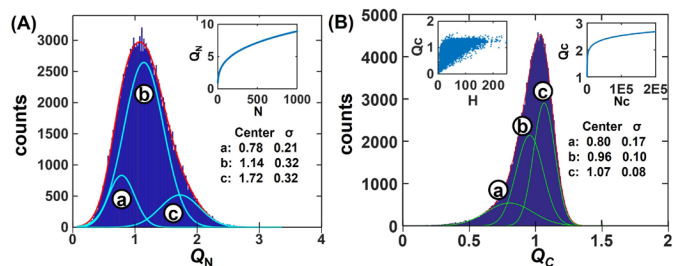
Figure 2: (A) Histogram of Q_N in top 2% scientists fitted with three Gaussian peaks. Inset shows H = N curve. (B) The distribution of Q_C fitted with three Gaussian peaks. Insets show the scattered plot of Q_C vs H (left) and the H = (Nc)^{0.5} curve (the maximum H value for a particular Nc , right).
