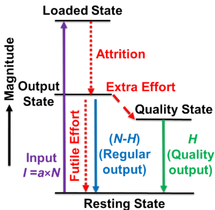
Figure 5: The M-C diagram of publication states. N and H depict the number of publications and h -index, respectively. “ I ” represents the total input whereas “ a ” depicts a proportionality factor.
