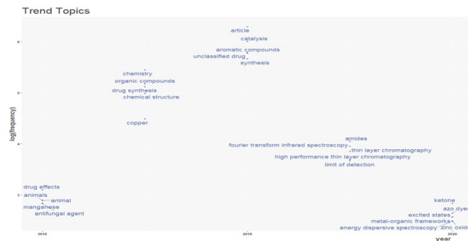
Figure 11: Trending Topics in Indian Chemistry research during 2016-2020.
