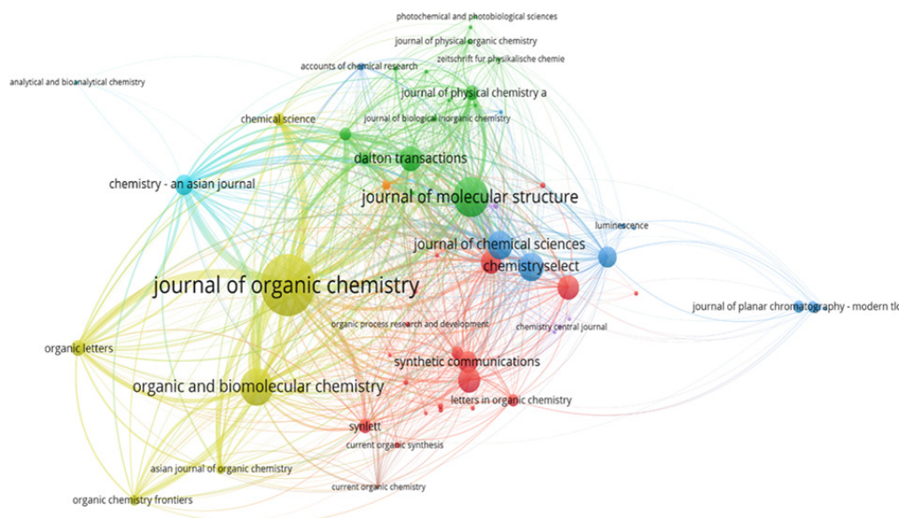
Figure 7: Bibliographic Coupling of Prolific Journals.
