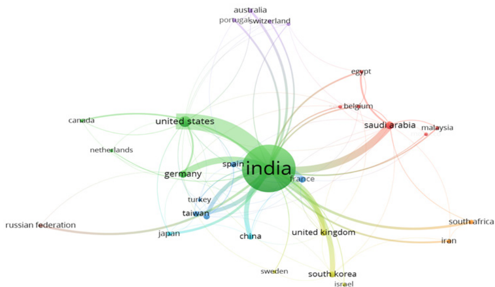
Figure 6: Network Visualization of co-authorship of countries.
