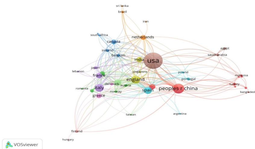
Figure 7: Countries co-authorship network. Notes: Minimum number of documents of a country is 4 and minimum number of citations of a country is 2. 45 documents and 6 clusters meet the threshold. The largest set of connected documents consists of 44 documents. Node=country, size of the node=document.
